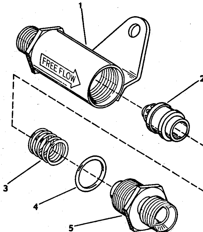
Exploded View - In-Line Check Valve
